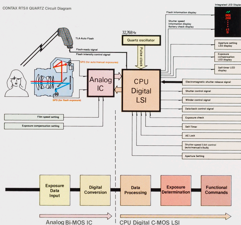
CONTAX RTSII QUARTZ Circuit Diagram
